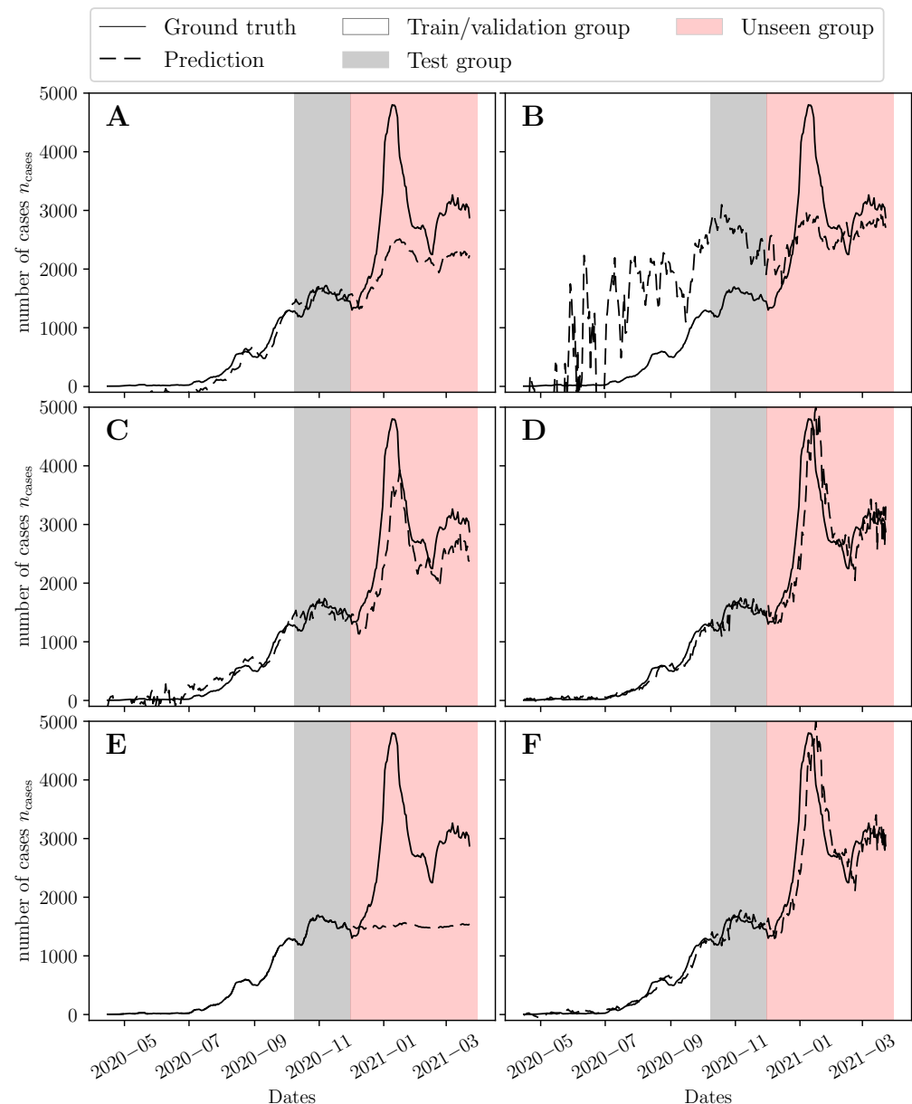
Figure 6. Predicted 7-day rolling average of daily number of cases on the unseen data set using (A) the sequence-to-sequence (S2S) model, (B) the stacked LSTM (SEQ), (C) The feedforward neural network (DNN), (D) The support vector machine regression (SVR) model, (E) The gradient boosting machine (GBM), and (F) the polynomial regression (OLS) model. All models were tuned using the validation error of the discovery set. The grey shaded region represents the test data set (Group 2) used to test the models' performance. The models were retrained using both the discovery and test data sets and subsequently used to infer the number of cases in the unseen data set (the red shaded region).
