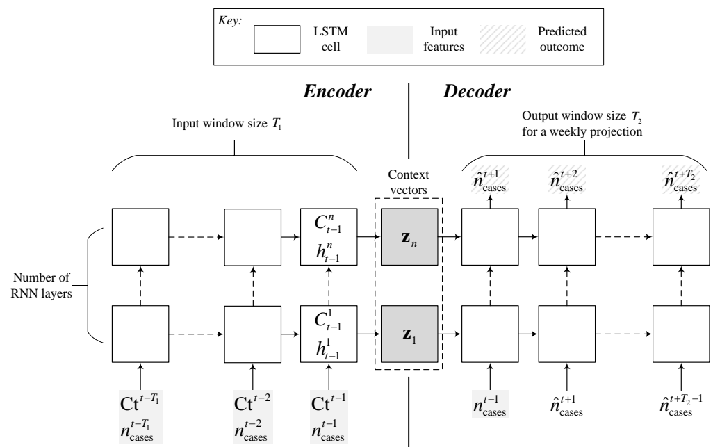
Figure 2. Structure of the sequence-to-sequence (S2S) model used for now-casting the weekly number of cases. The left side of the network is the encoder that uses past information on Ct and the number of cases to create context vectors used to initialize the hidden and cell states of the decoder LSTM cells.
