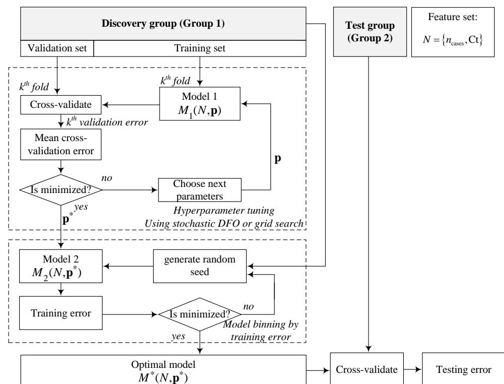
Figure 3. Cross-validation and hyperparameter determination scheme for model development. Following the discovery group (Group 1), the inner loop tuned the model’s hyperparameters by minimizing the average k -fold cross-validation error using a stochastic direct search algorithm or a grid search. The second loop (following tuning) generates several models randomly and bins them by training error. The best model with the lowest training error is tested on the test group to obtain the testing error.
