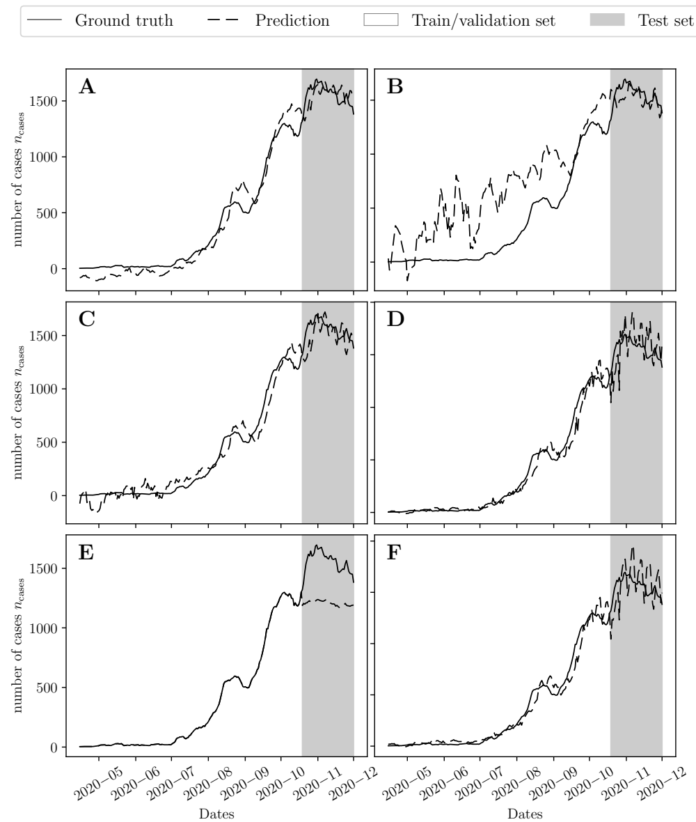
Figure 5. Predicted 7-day rolling average of daily number of cases on the unseen data set using (A) the sequence-to-sequence (S2S) model, (B) the stacked LSTM (SEQ), (C) The feedforward neural network (DNN), (D) The support vector machine regression (SVR) model, (E) The gradient boosting machine (GBM), and (F) the polynomial regression (OLS) model. All models were tuned using the cross-validation error of the discovery set. The grey shaded region represents the test data set (Group 2) used to test the models' performance.
